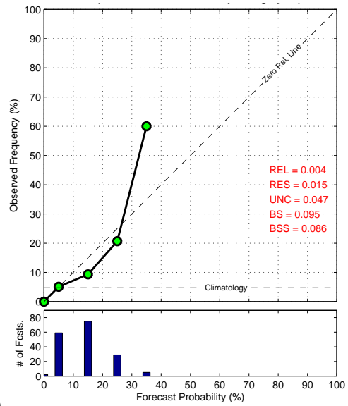
Figure 4.19. KLF1 GEPS reliability diagrams for 6 hr precipitation: a: 48 hr forecast. b: 240 hr forecast.
